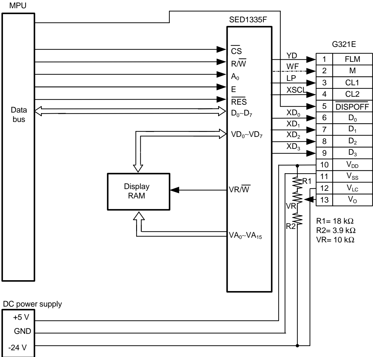
Figure 12 Interface Circuit With SED1335F
