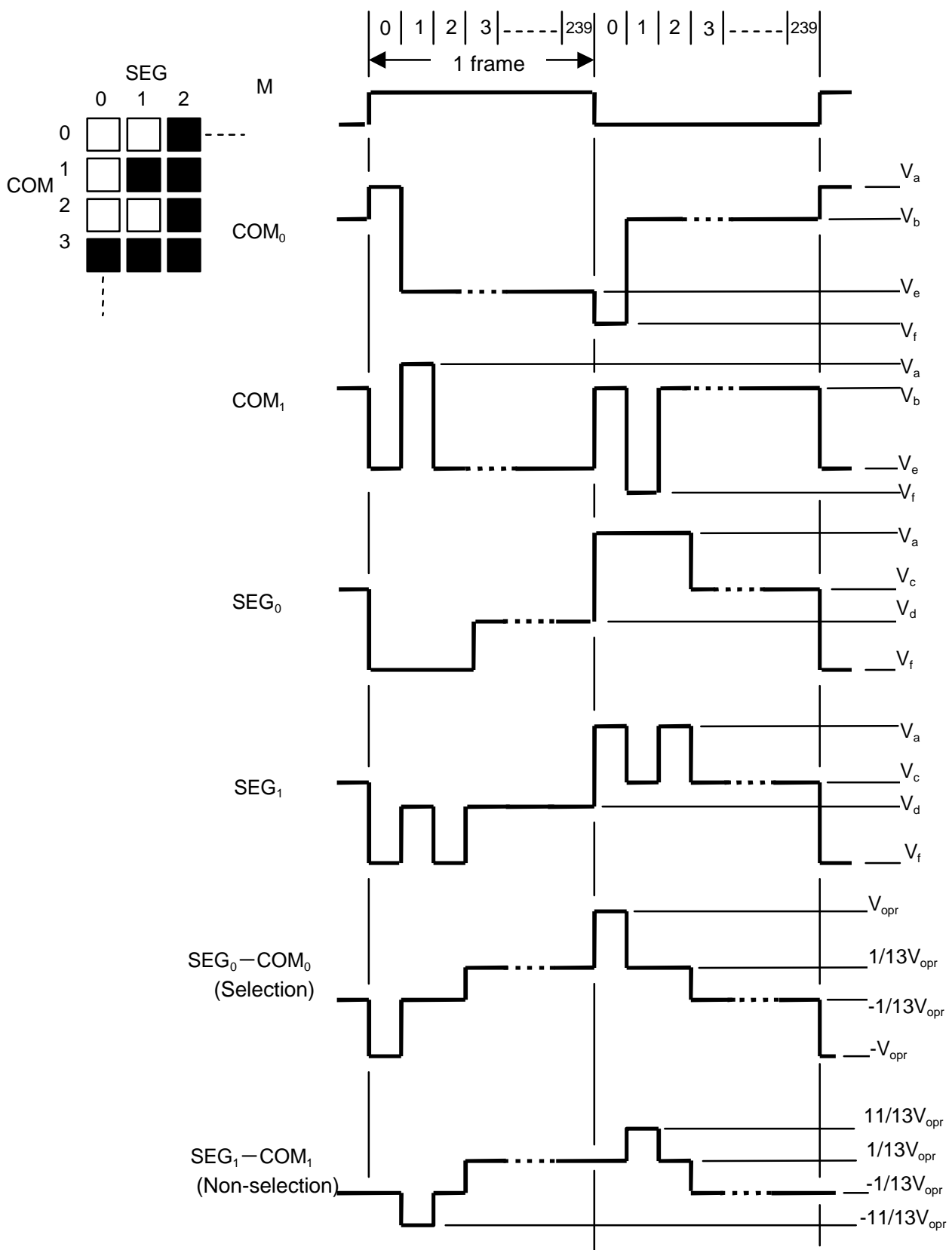
Figure 2 Drive Waveform
