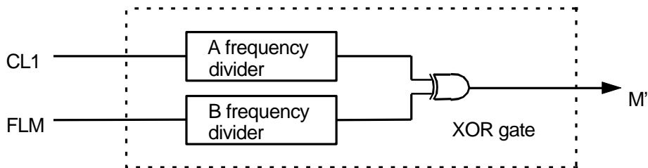
Figure 7 M' Generation Circuit
