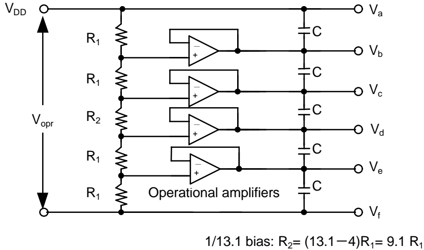
Figure 6 Bias Voltage Generation Circuit
