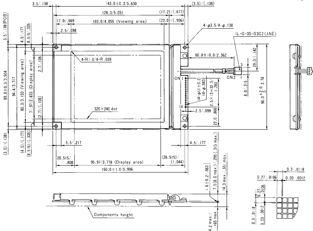
Figure 1 Dimensions
