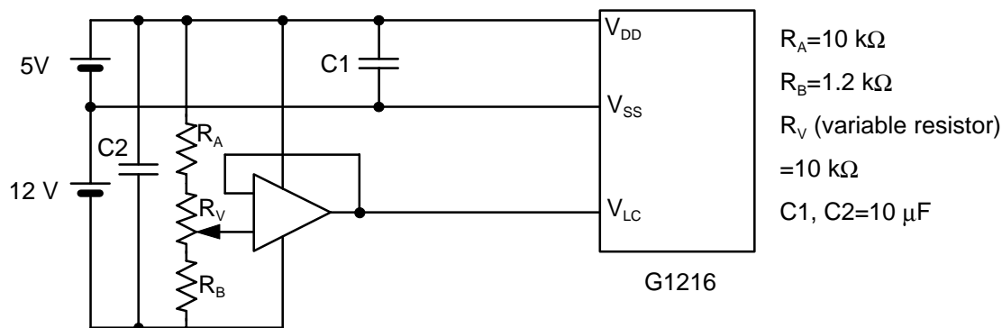
Figure 10 Contrast Adjustment
