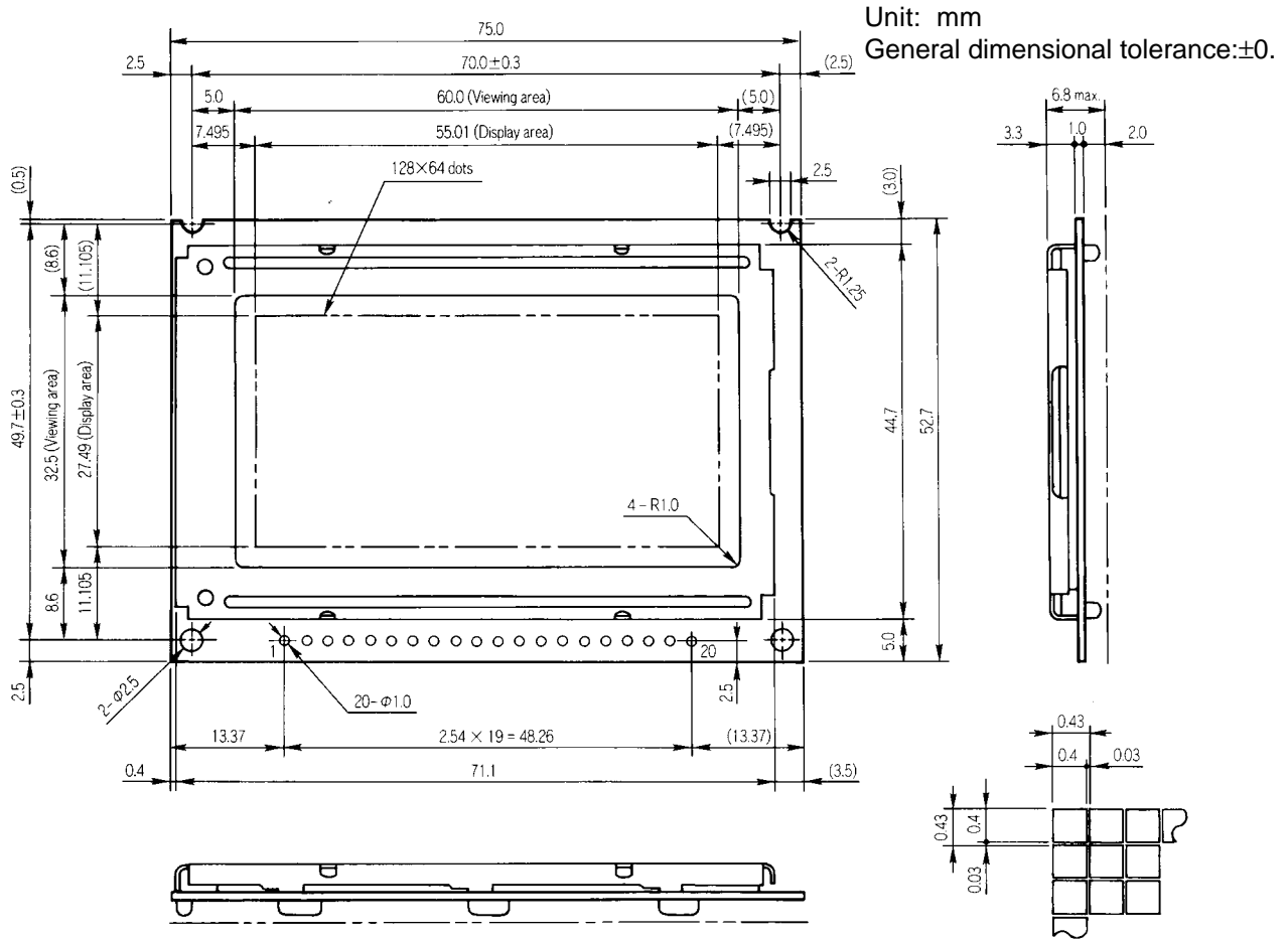
Figure 1 Dimensions
